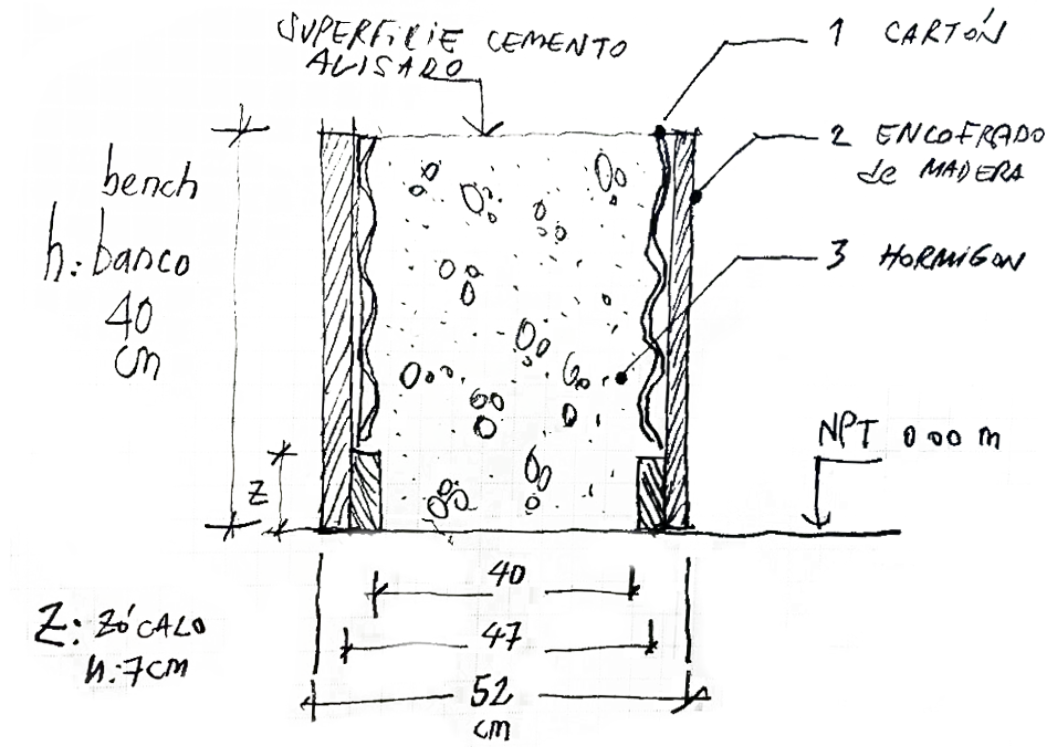
Sketch of the formwork.
